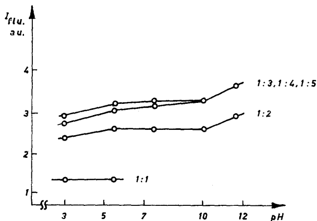
Fig. 2. The intensity of the fluorescence band at \lambda = 577 nm for Dy(III):NTA molar ratios 1:1, 1:2, 1:3, 1:4 and 1:5 as a function of the pH
