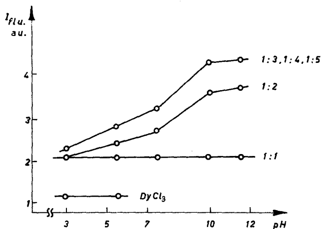
Fig. 1. The intensity of the fluorescence band at \lambda = 577 nm for Dy(III):EDTA molar ratios 1:1, 1:2, 1:3, 1:4 and 1:5 as a function of the pH
