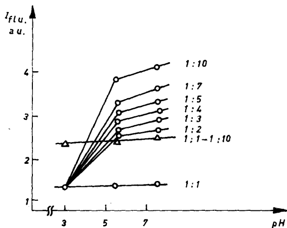
Fig. 4. The intensity of the fluorescence bands at \lambda = 590 and 615 nm for Eu:AA = 1:1—1:10 as a function of the pH
