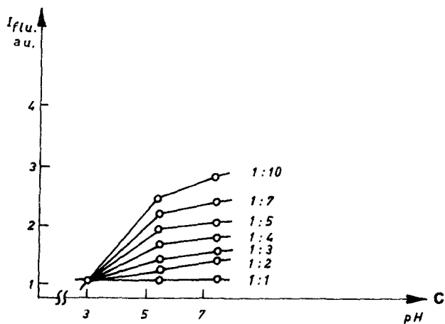
Fig. 3. The intensity of the fluorescence bands of Gd, Tb and Dy complexes with acetic acid as a function of the pH : a at \lambda = 312 nm for Gd:AA = 1:1–1:10; b at \lambda = 545 nm for Tb:AA = 1:1–1:10; c at \lambda = 577 nm for Dy:AA = 1:1–1:10
